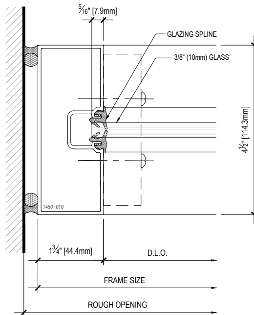
P2 PLAN -JAMB DETAIL - 3/8" GLASS INFILL
