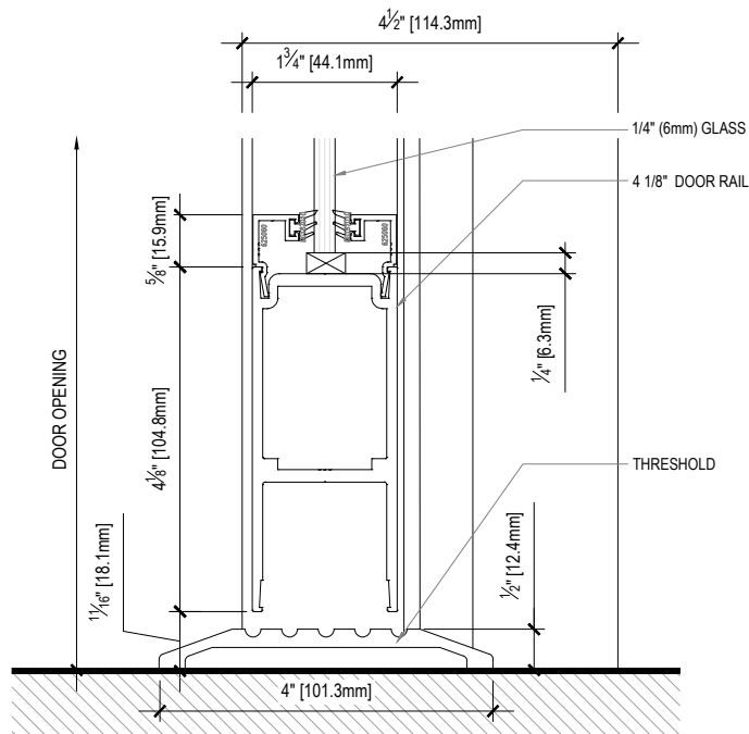
S17 SECTION -DOOR SILL DETAIL - 1/4" GLASS INFILL
