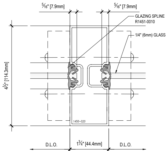
P3 PLAN - VERTICAL INTERMEDIATE MULLION DETAIL - 1/4" GLASS INFILL
