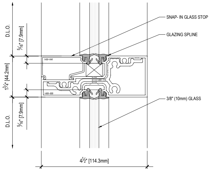
S6 SECTION -HORIZONTAL TRANSOM DETAIL - 3/8" GLASS INFILL
