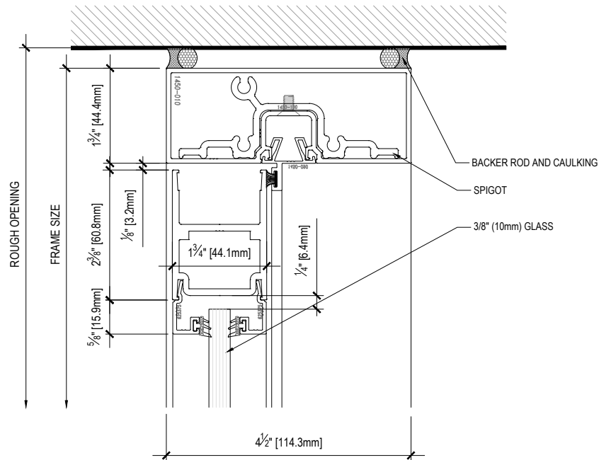
S14 SECTION -HEAD DETAIL WITH 218 DOOR SYSTEM - 3/8" GLASS INFILL
