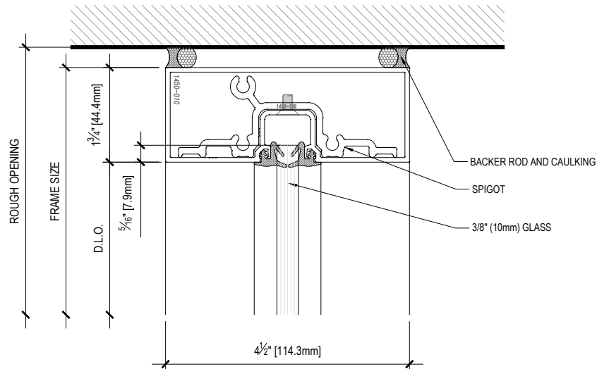
S8 SECTION -HEAD DETAIL - 3/8" GLASS INFILL
