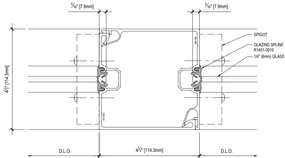
P5 PLAN - BOX INTERMEDIATE DETAIL - 1/4" GLASS INFILL
