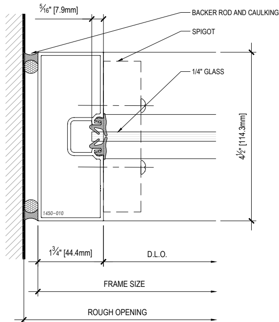
P1 PLAN -JAMB DETAIL - 1/4" GLASS INFILL
