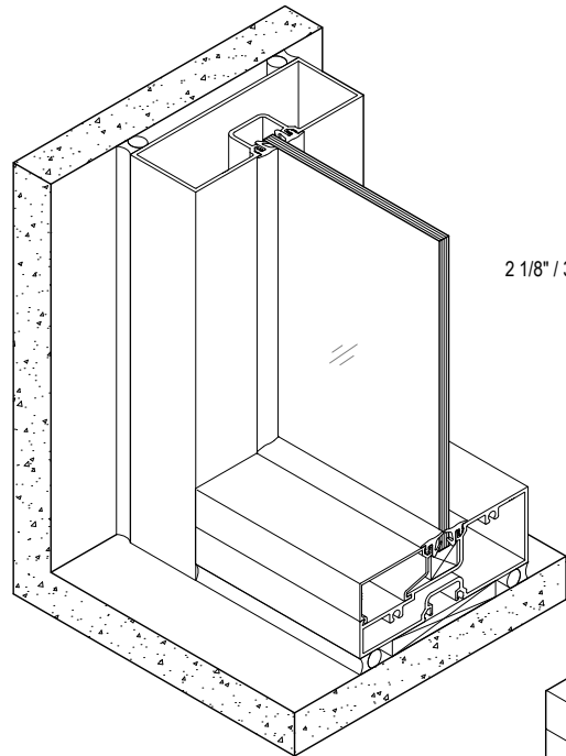
2 ISOMETRIC VIEW (TYPICAL JAMB)
