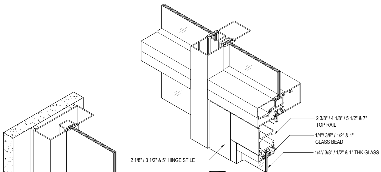
1 ISOMETRIC VIEW (TOP RAIL)
