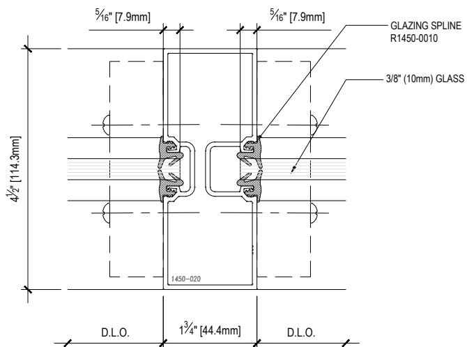
P4 PLAN - VERTICAL INTERMEDIATE MULLION DETAIL - 3/8" GLASS INFILL
