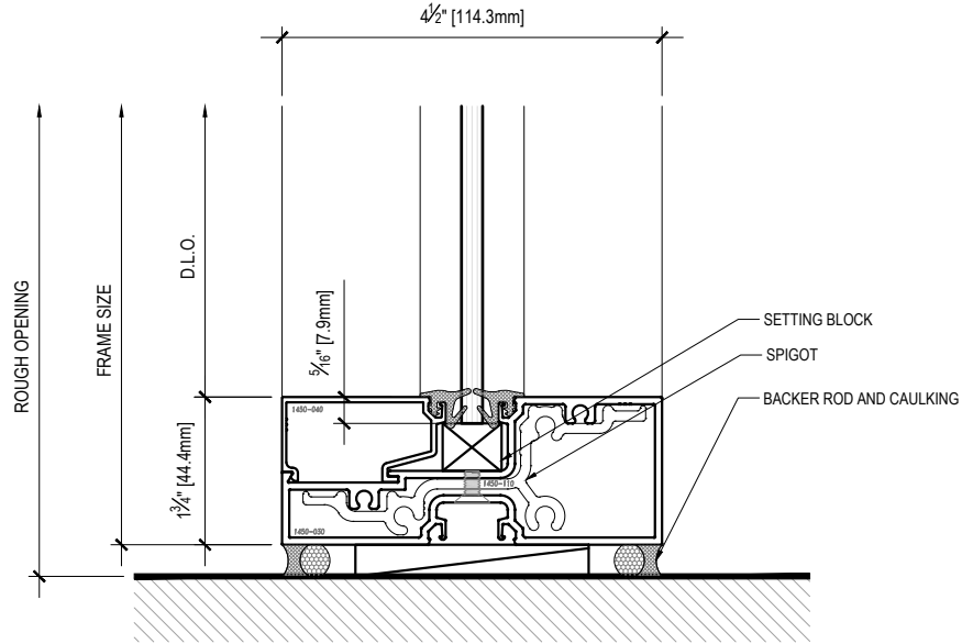
S1 SECTION - SILL DETAIL - 1/4" GLASS INFILL
