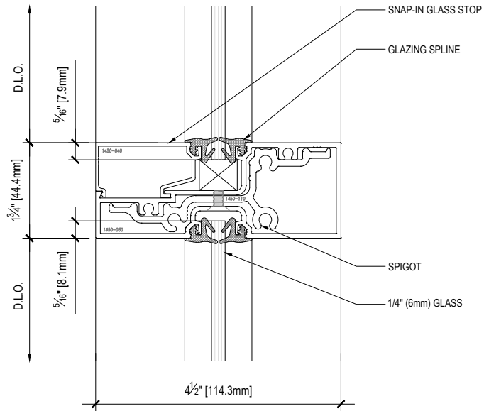
S5 SECTION -HORIZONTAL TRANSOM DETAIL - 1/2" GLASS INFILL
