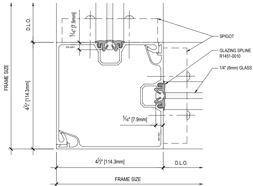
P7 PLAN - 90° CORNER DETAIL - 1/4" GLASS INFILL
