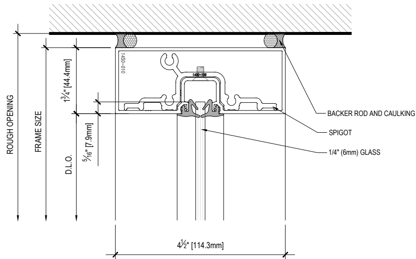
S7 SECTION -HEAD DETAIL - 1/4" GLASS INFILL
