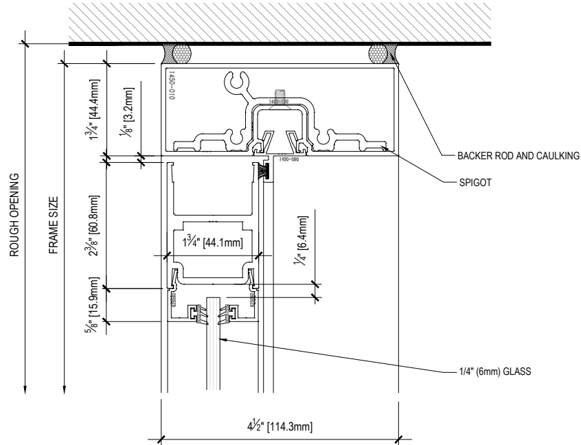
S13 SECTION -HEAD DETAIL WITH 218 DOOR SYSTEM - 1/4" GLASS INFILL
