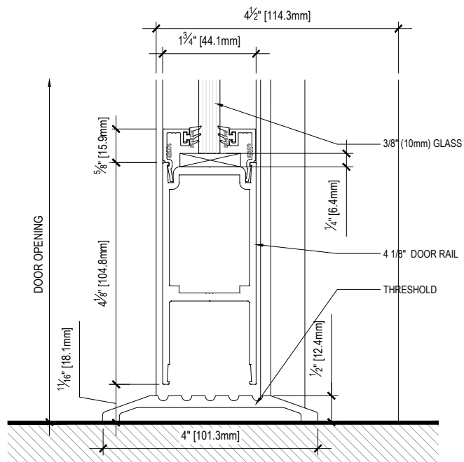
S18 SECTION -DOOR SILL DETAIL - 3/8" GLASS INFILL
