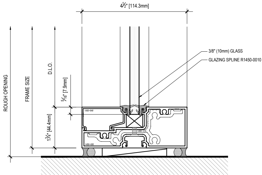
S2 SECTION - SILL DETAIL - 3/8" GLASS INFILL
