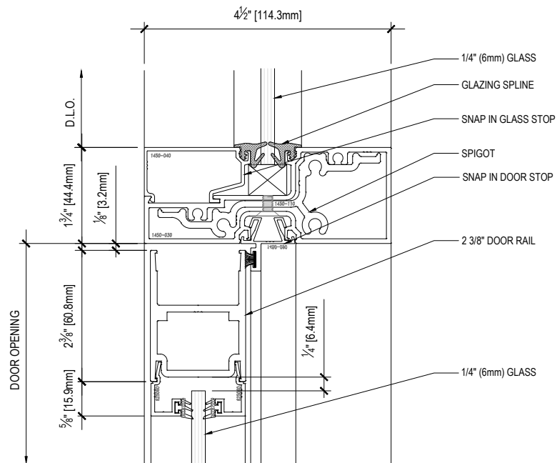
S15 SECTION -INTERMEDIATE HORIZONTAL DETAIL - 1/4" GLASS INFILL
