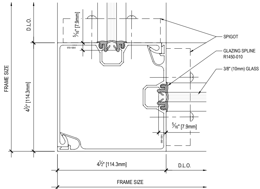
P8 PLAN - 90° CORNER DETAIL - 3/8" GLASS INFILL
