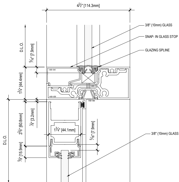
S16 SECTION -INTERMEDIATE HORIZONTAL DETAIL - 3/8" GLASS INFILL
