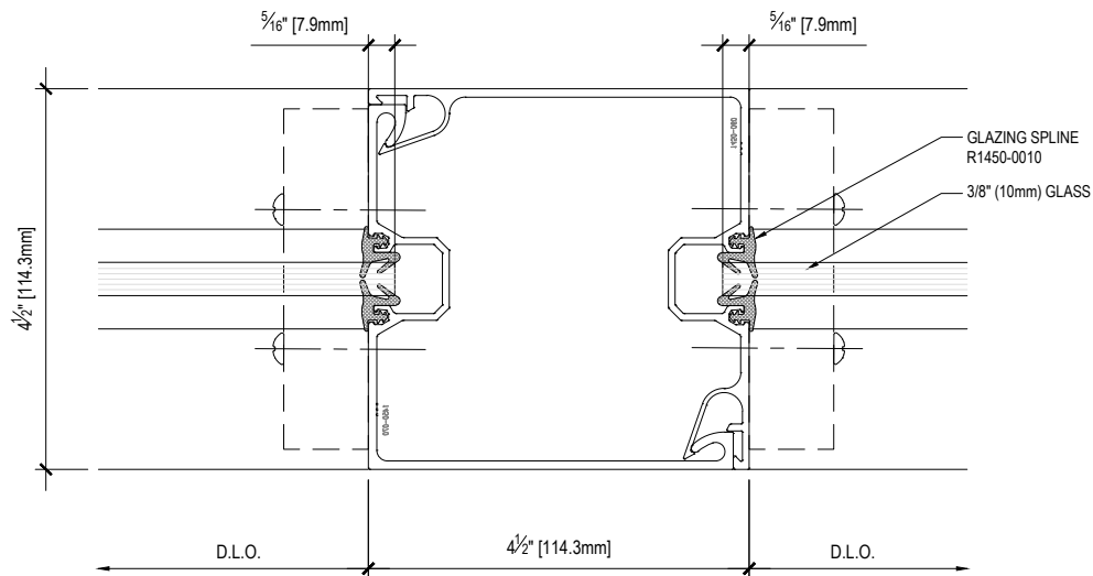
P6 PLAN - BOX INTERMEDIATE DETAIL - 3/8" GLASS INFILL
